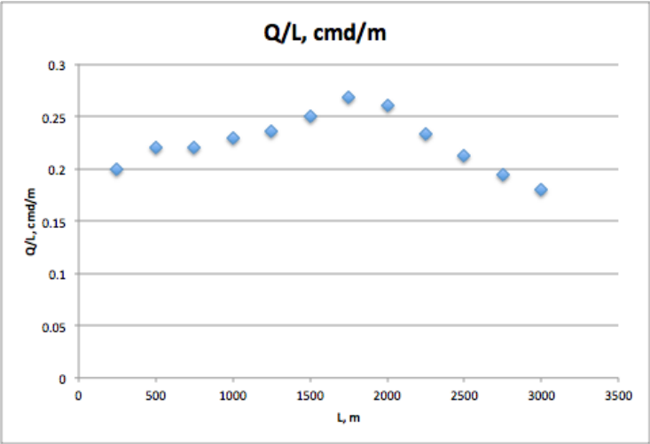
Fig. 1. Specific Flowrate Q/L vs Horizontal Length L
