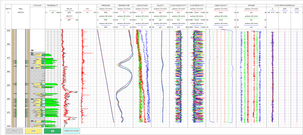
Fig. 4. PLT in shut-in water injector
