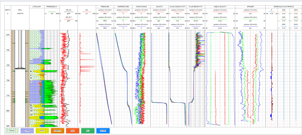
Fig. 2. PLT in shut-in oil producer
