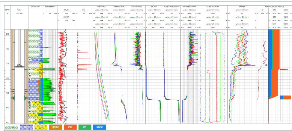
Fig. 1. PLT in flowing oil producer
