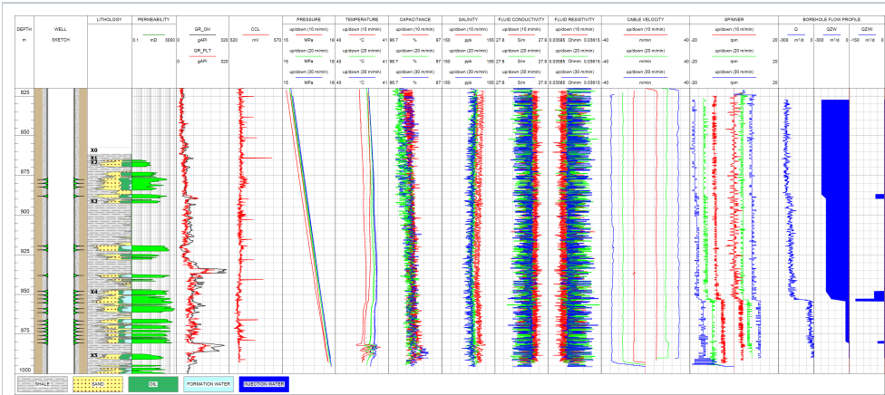
Fig. 3. PLT in flowing water injector
