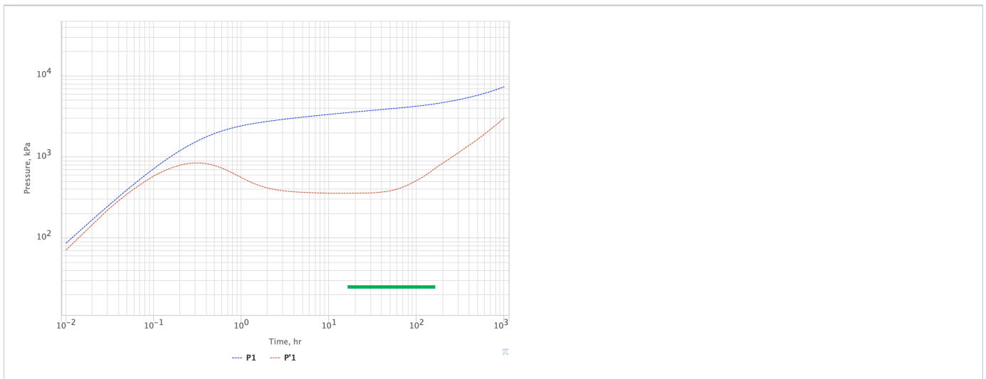
Fig. 2. Example of the fault impact on radial flow which may lead to the wrong estimation of reservoir transmissibility.
