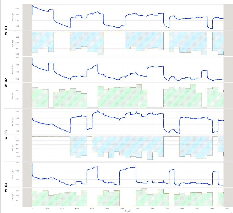
Fig. 1. Production/Injection History
